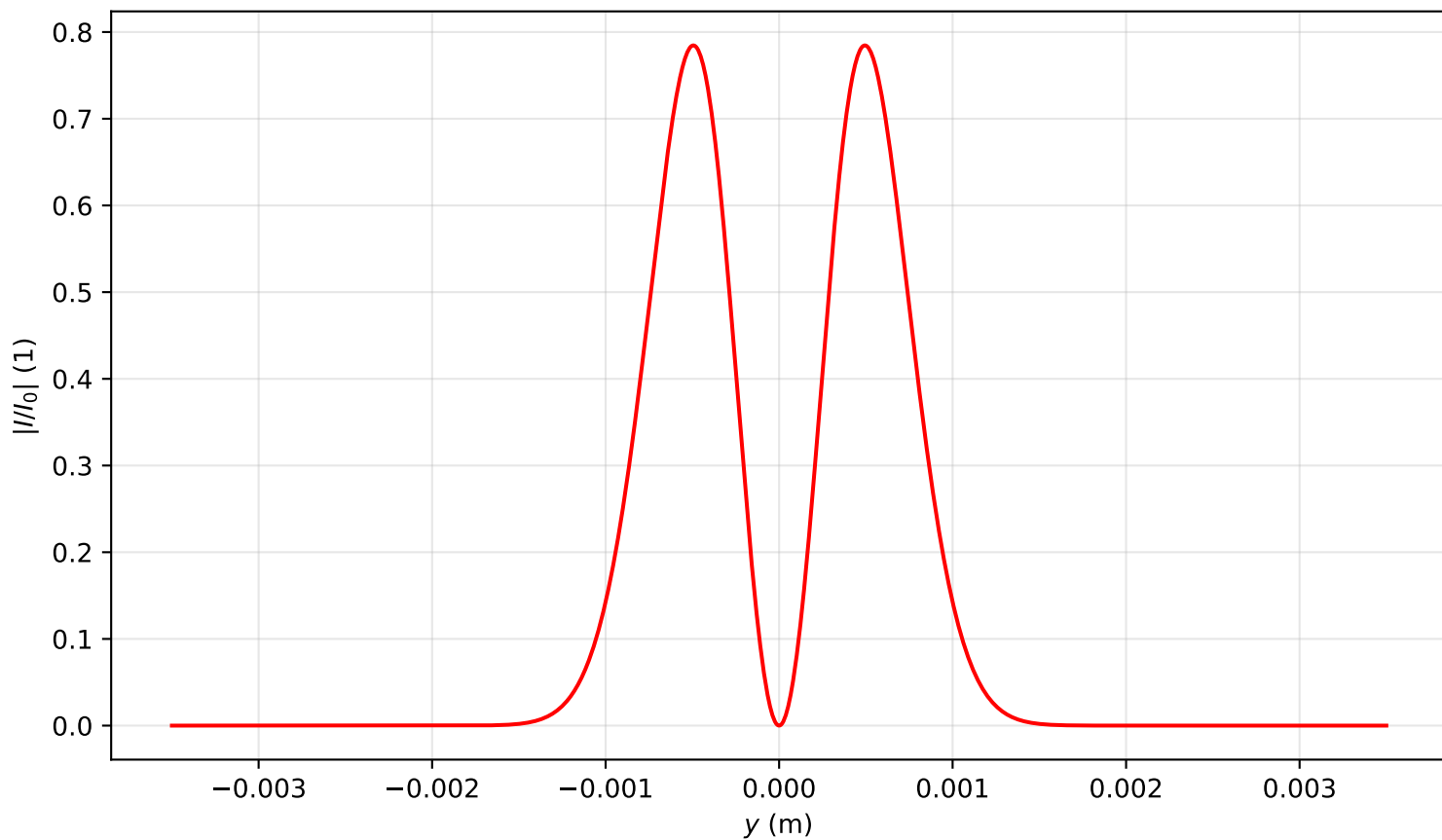
Intensity profile I(x=0, y, z=0.080)/I_0 , P_{in}=4.0P_{cr} , artificial time
